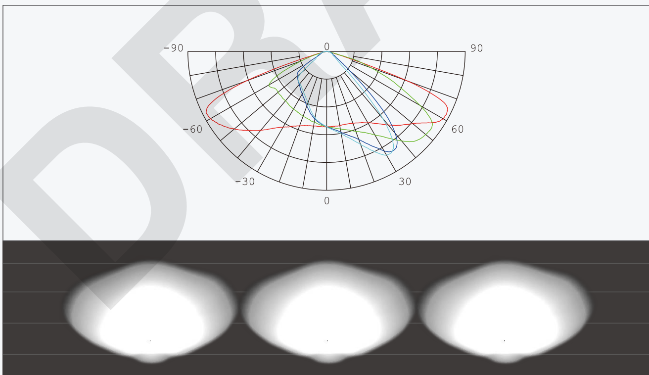
Type 3 FWHM 140° x70°
